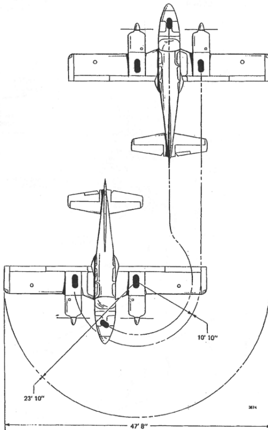
Figure 7-9. Minimum Turning Radius.
