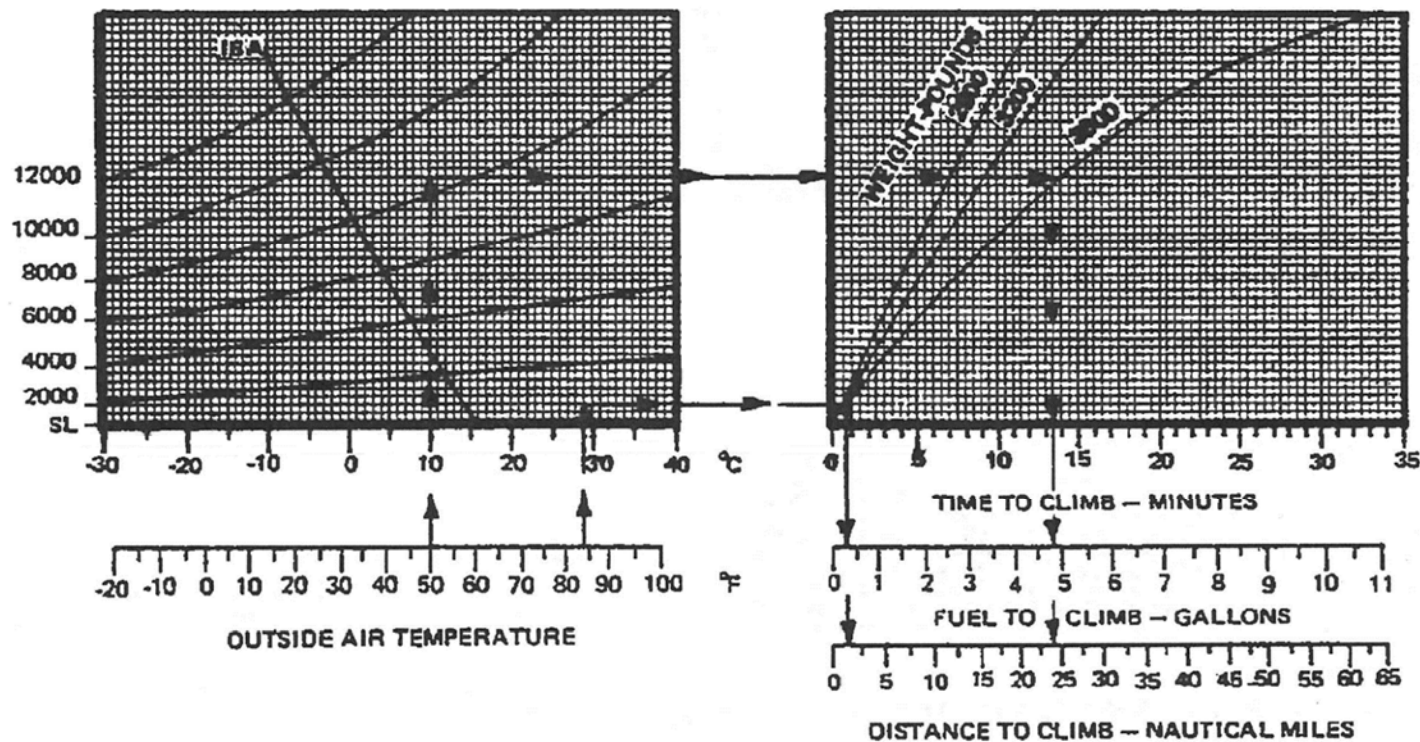
Figure 5-12. Time, Fuel and Distance to Climb (Cruise Climb).
