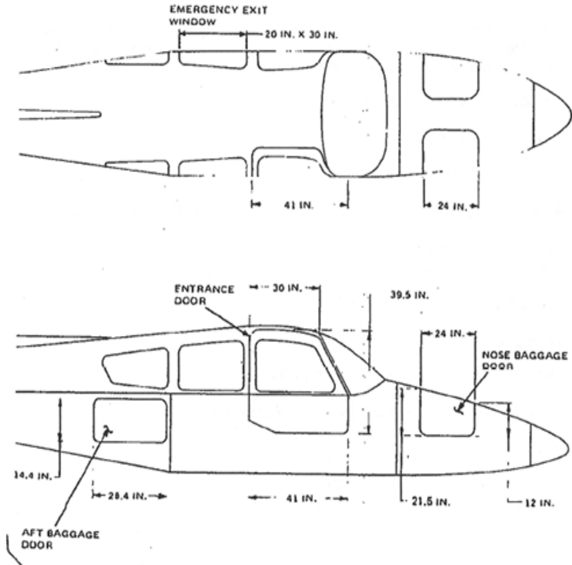
Figure 1-2. Cabin, Baggage and Entrance Dimensions.
