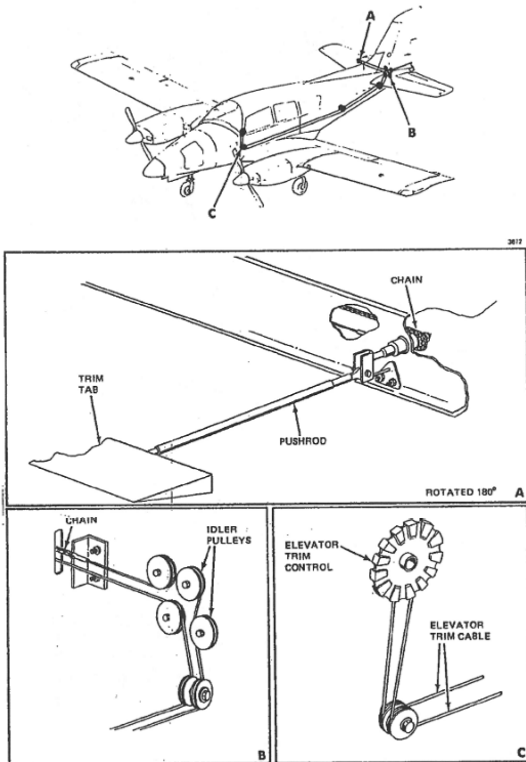
Figure 7-3. Elevator Trim System.
