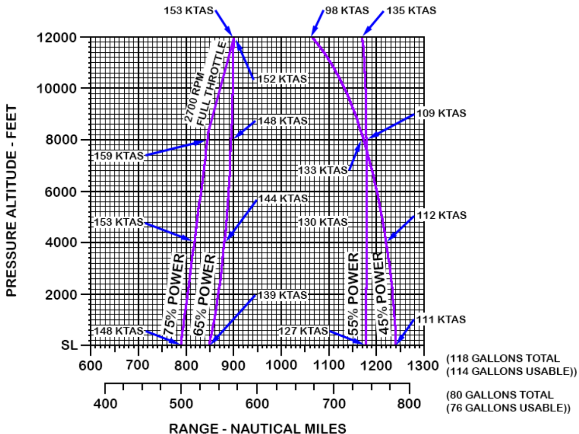
Figure 5-16. Range Profile.
