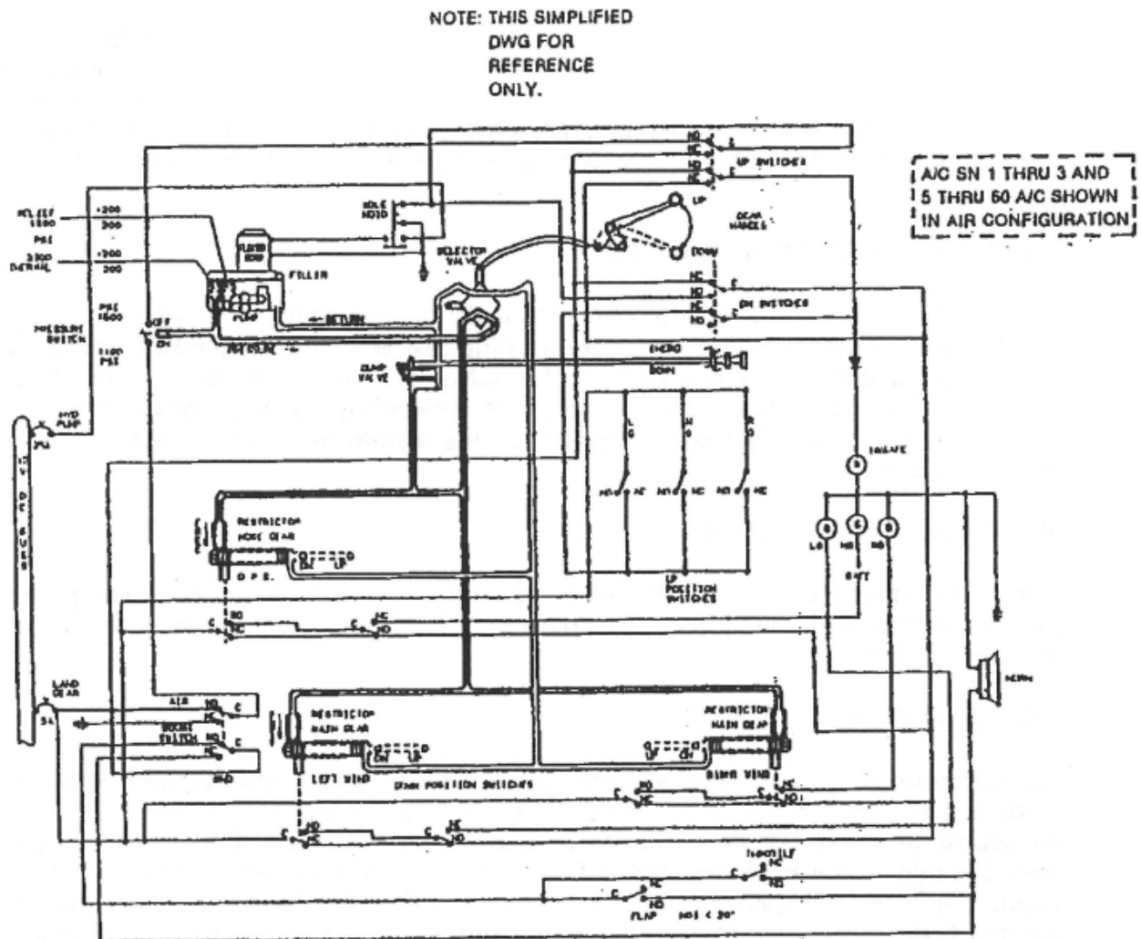
Figure 7-11. Hydraulic System Schematic (Gear Retracted).
