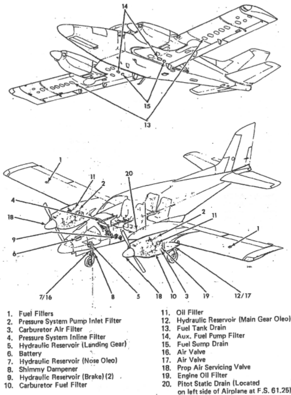
Figure 8-1. Servicing Points.
