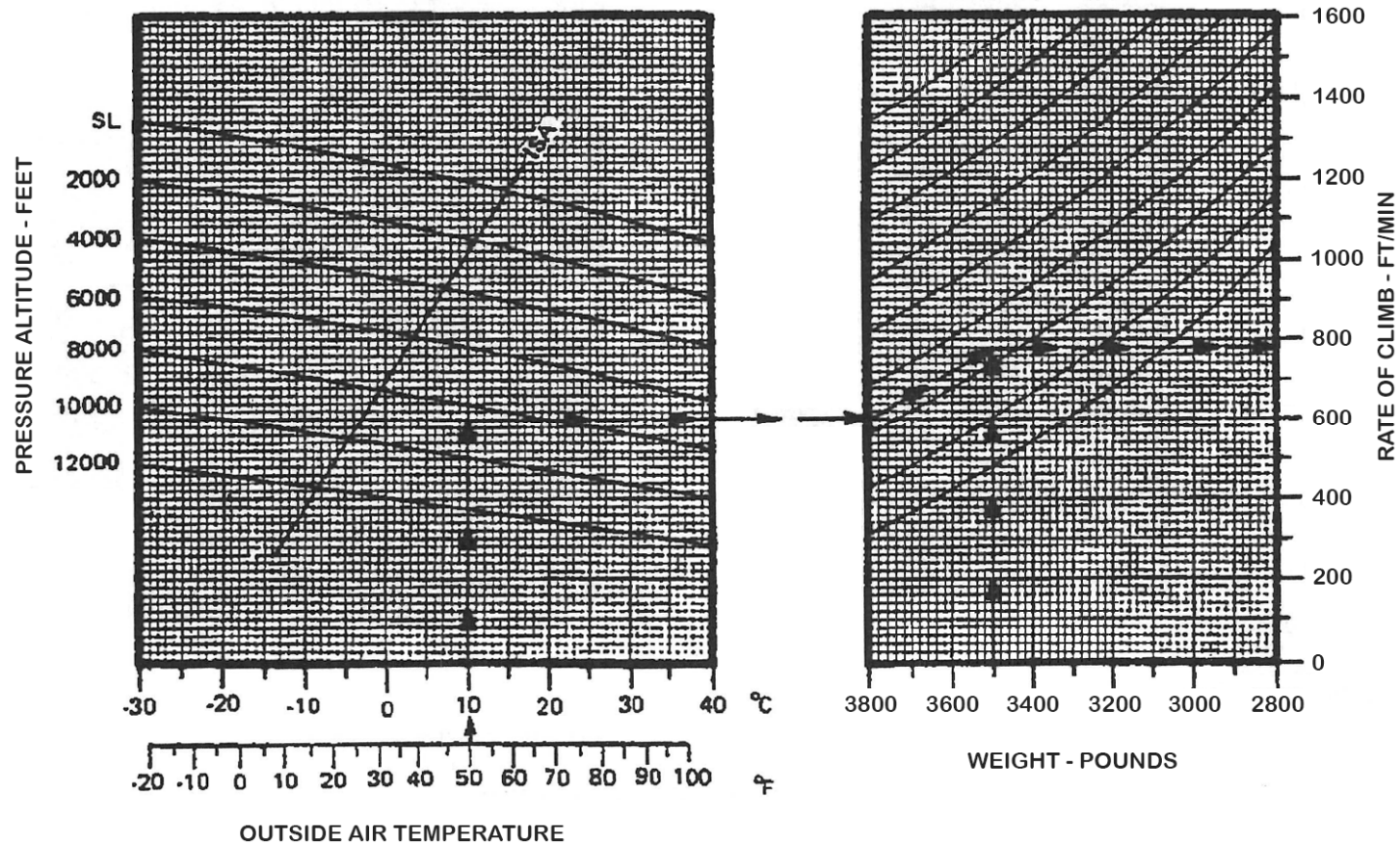
Figure 5-11. Climb – Two Engine (Maximum Climb).
