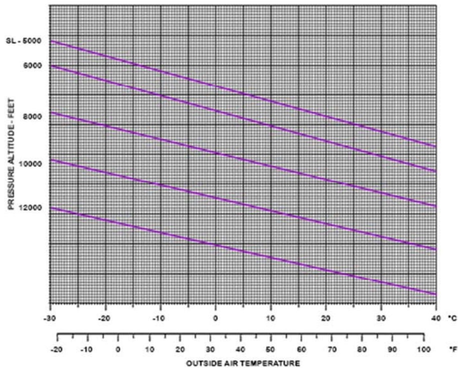
Figure 5-10. Climb – Two Engine (Cruise Climb).
