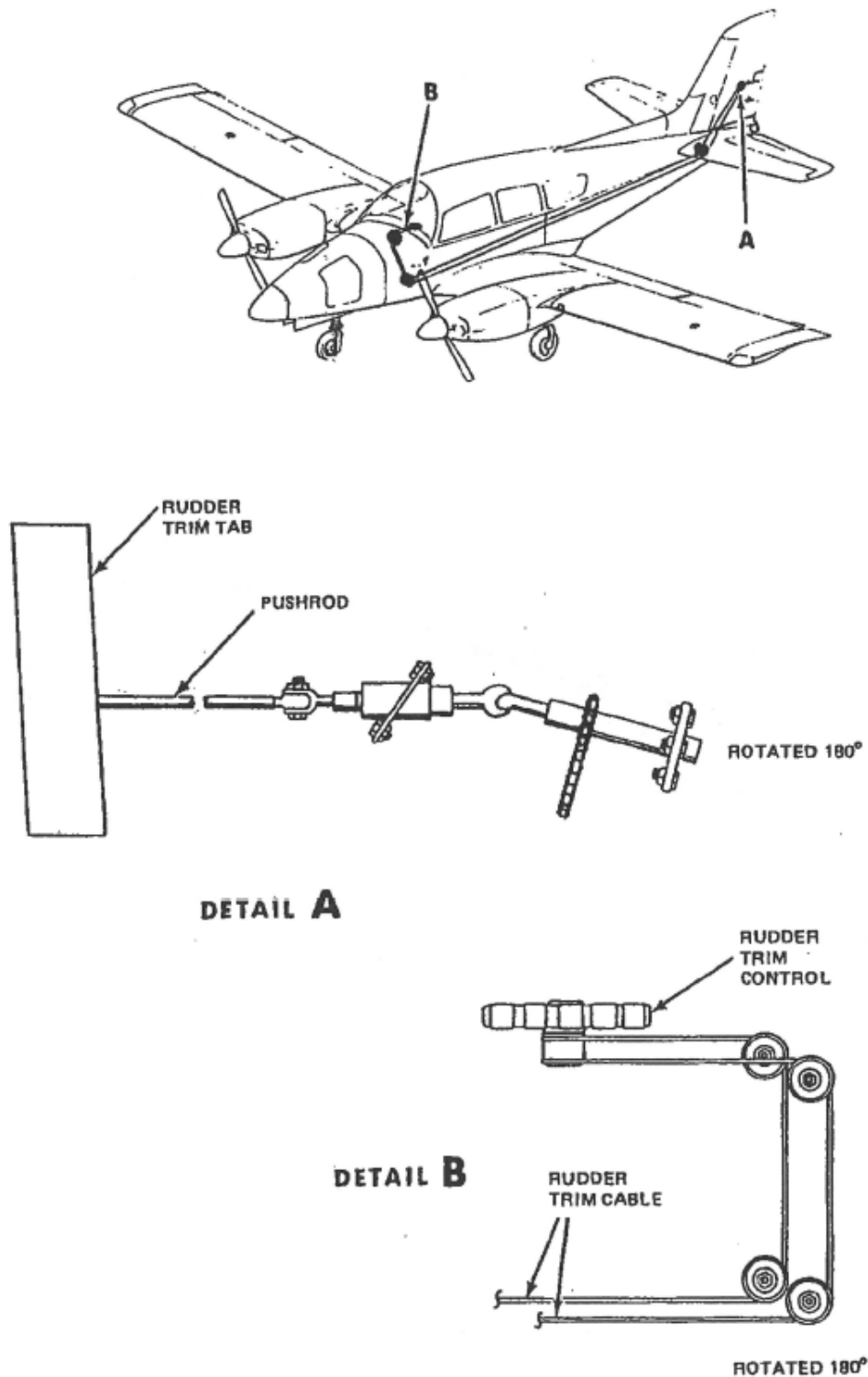
Figure 7-5. Rudder Trim System.
