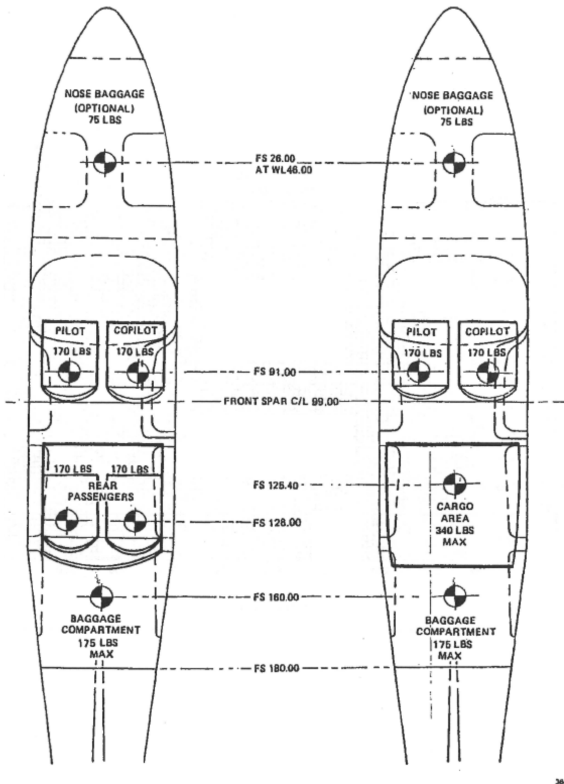
Figure 6-7. Seating – Cargo Arrangement and Center of Gravity Locations
