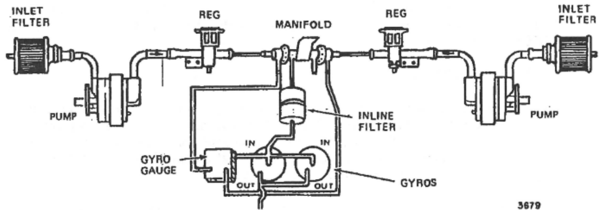
Figure 7-13. Pressure System Schematic.
