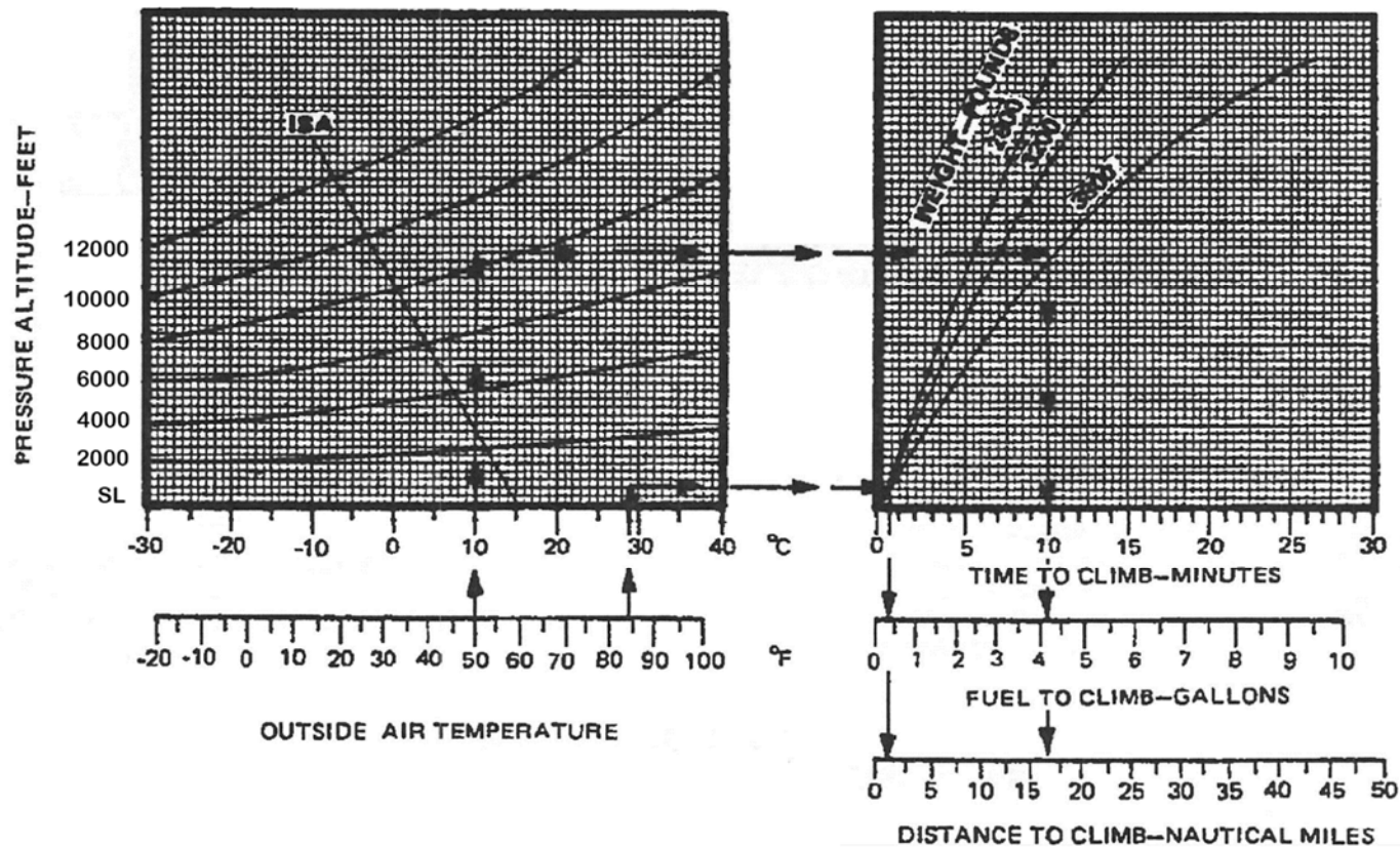
Figure 5-13. Time, Fuel and Distance to Climb (Maximum Climb).
