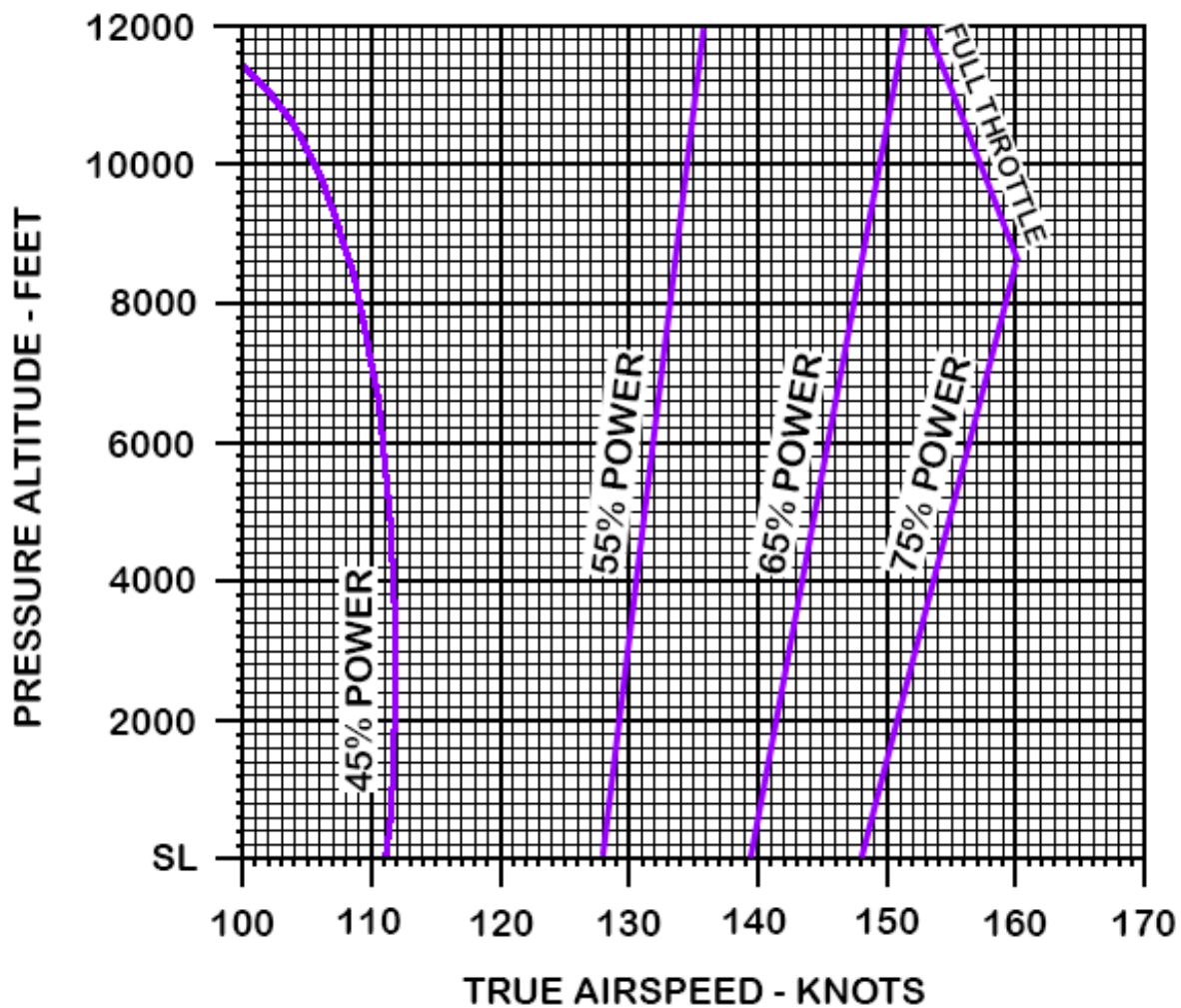
Figure 5-15. Cruise Speeds.
