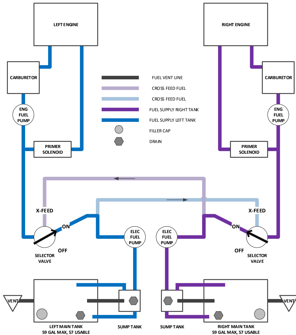
Figure 7-10. GA-7/Cougar Fuel System Schematic.
