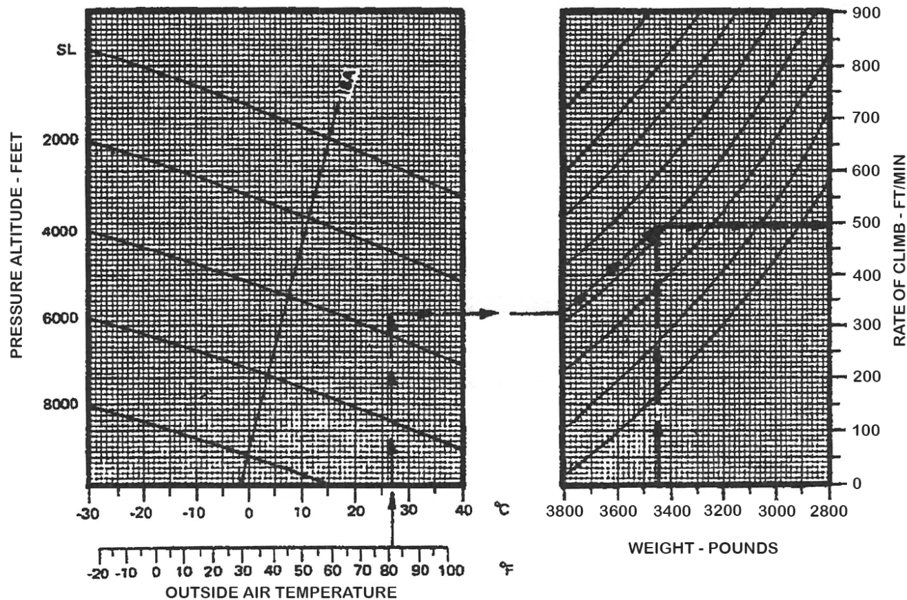
Figure 5-20. Climb – Balked Landing.
