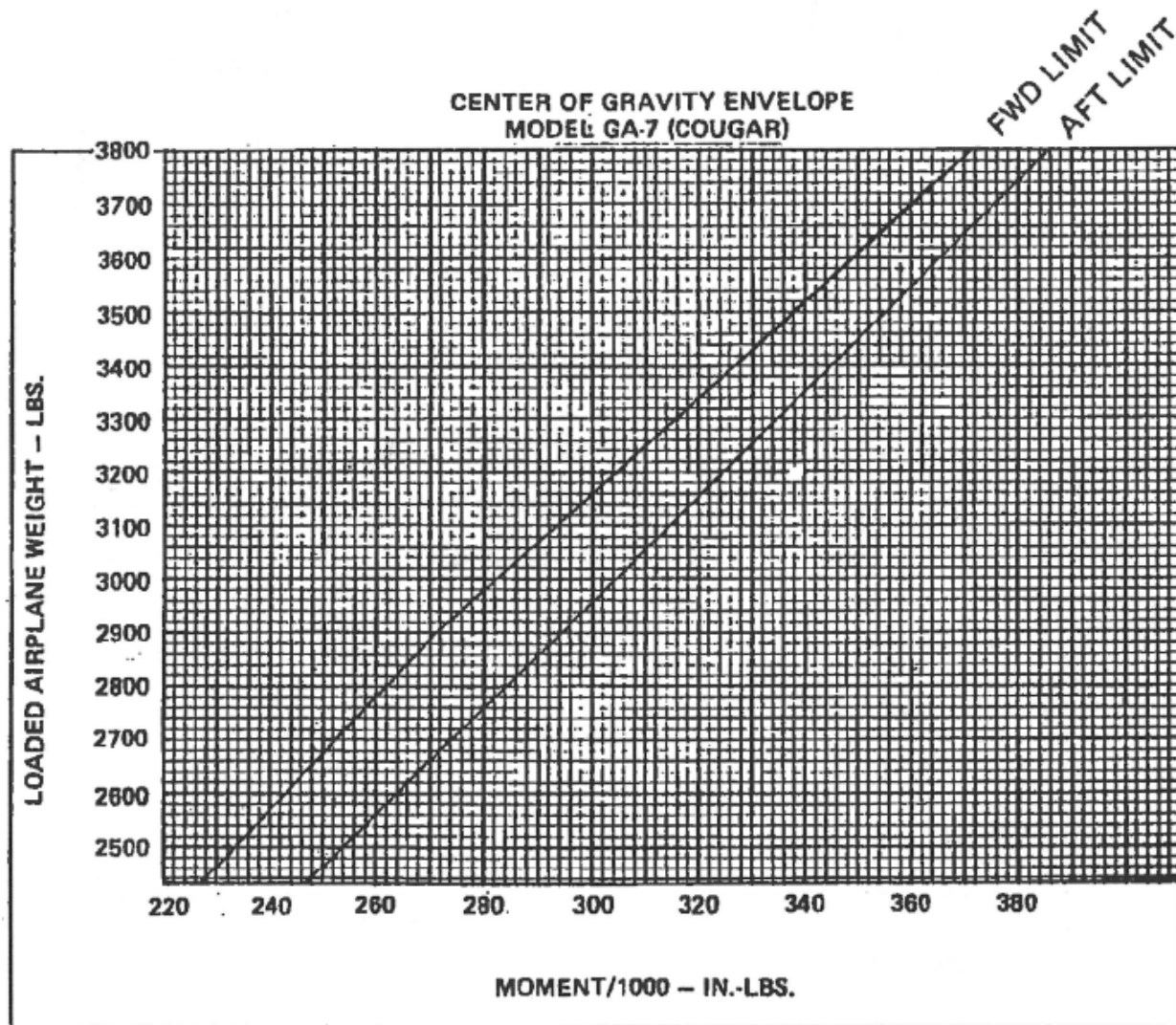
Figure 6-6. Center of Gravity Envelope
