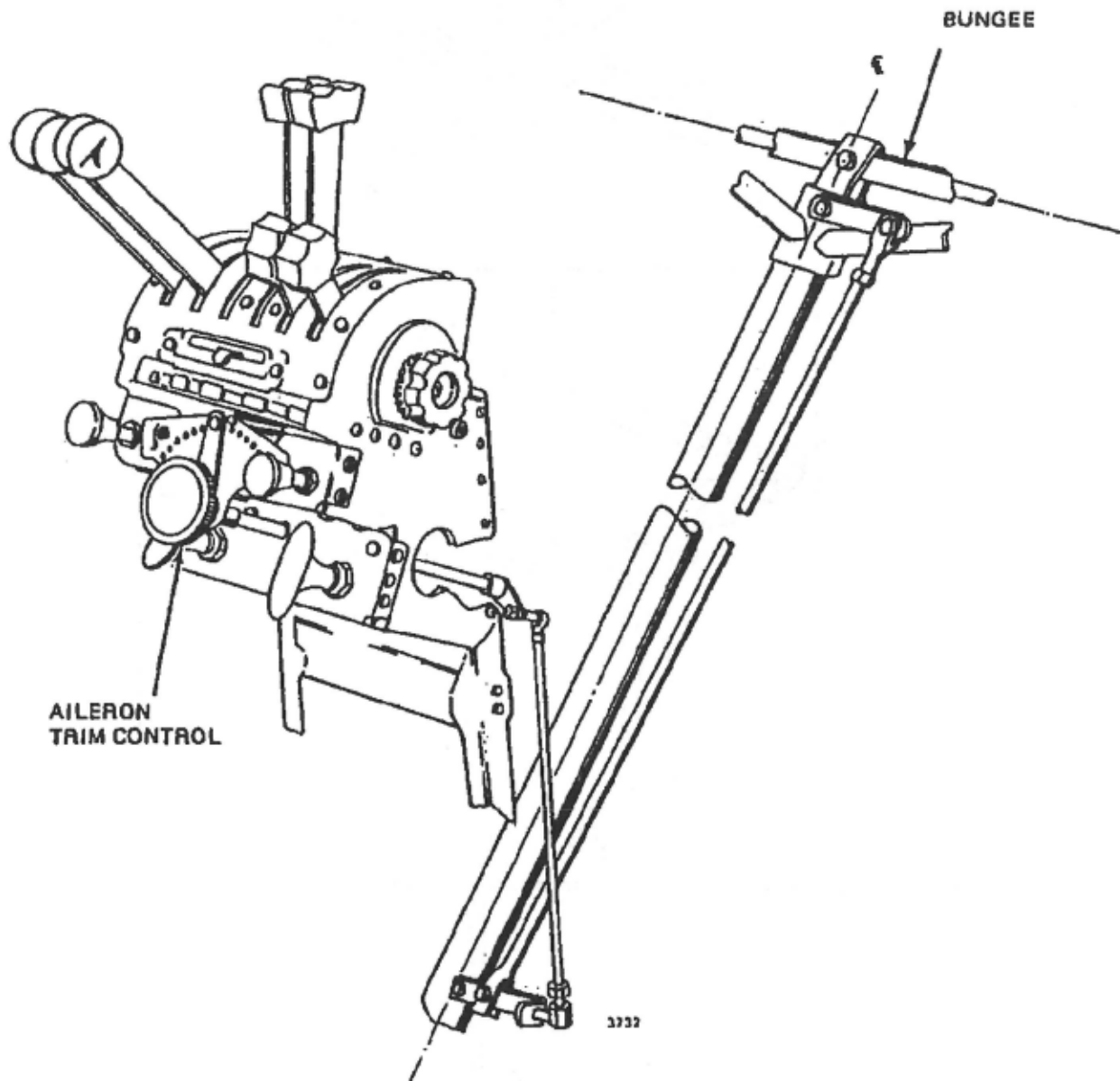
Figure 7-1. Aileron Control System (Sheet 2 of 2)
