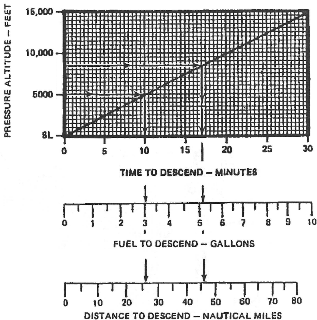
Figure 5-18. Time, Fuel and Distance to Descend.
