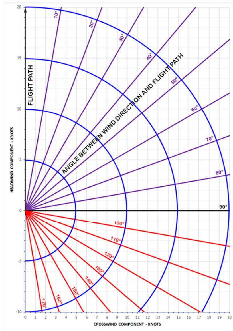
Figure 5-5. Crosswind Component Chart.
