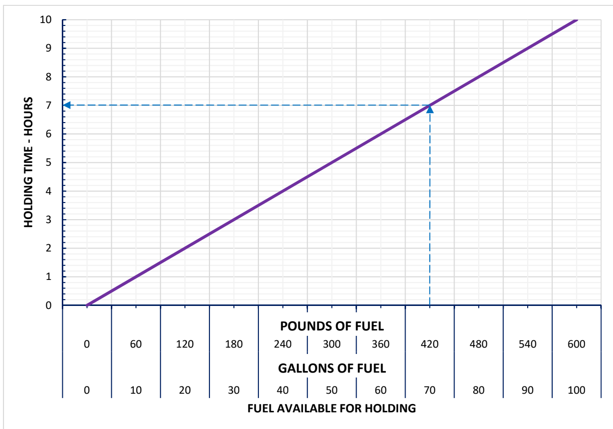
Figure 5-19. Holding Time.
