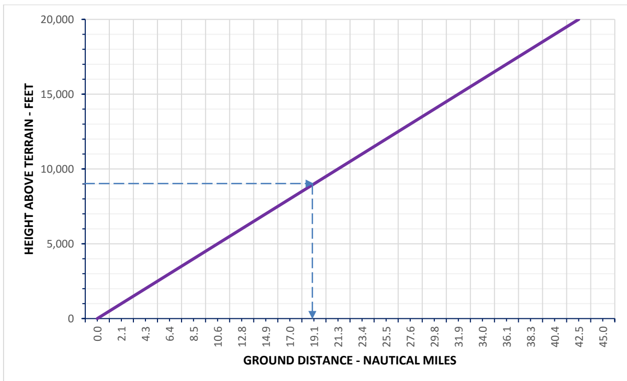
Figure 3-1. Maximum Glide.
