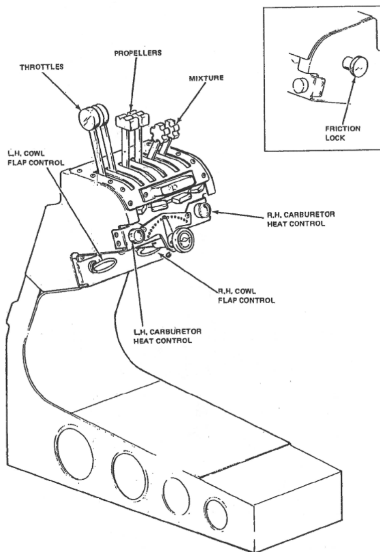
Figure 7-8. Engine Controls.
