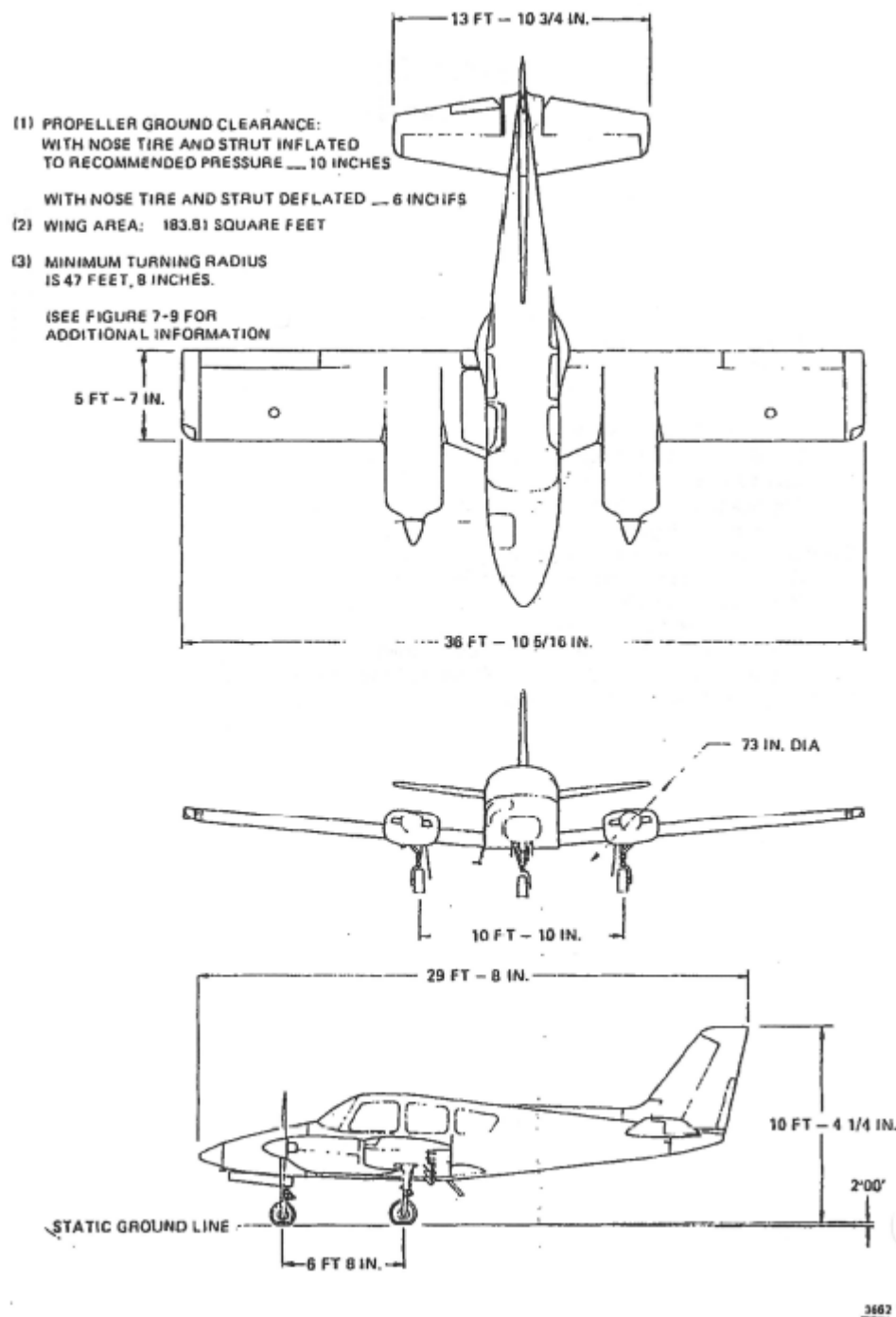
Figure 1-1. Three View.
