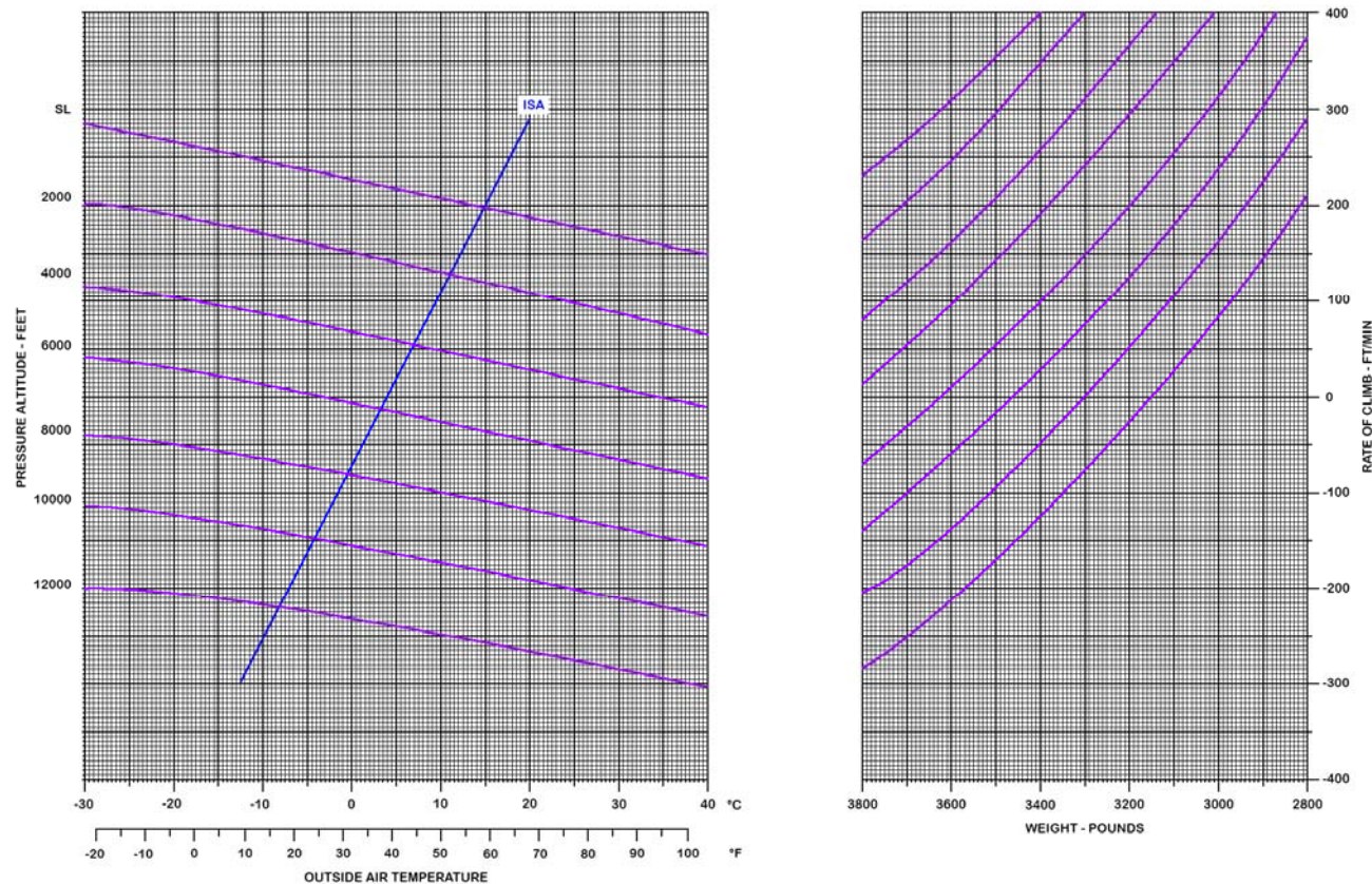
Figure 5-8. Climb – One Engine Inoperative.
