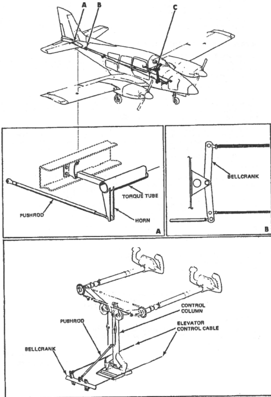
Figure 7-2. Elevator Control System.
