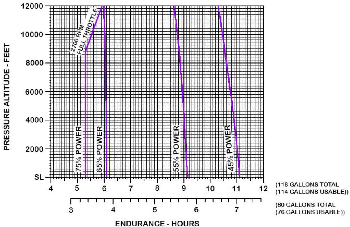
Figure 5-17. Endurance Profile.
