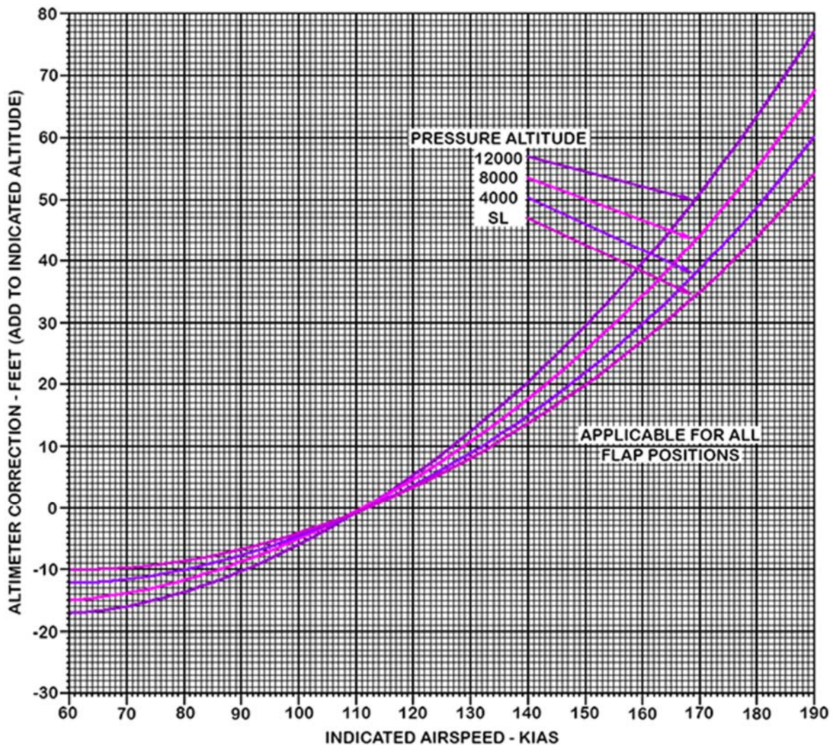
Figure 5-2. Altimeter Correction – Normal System
