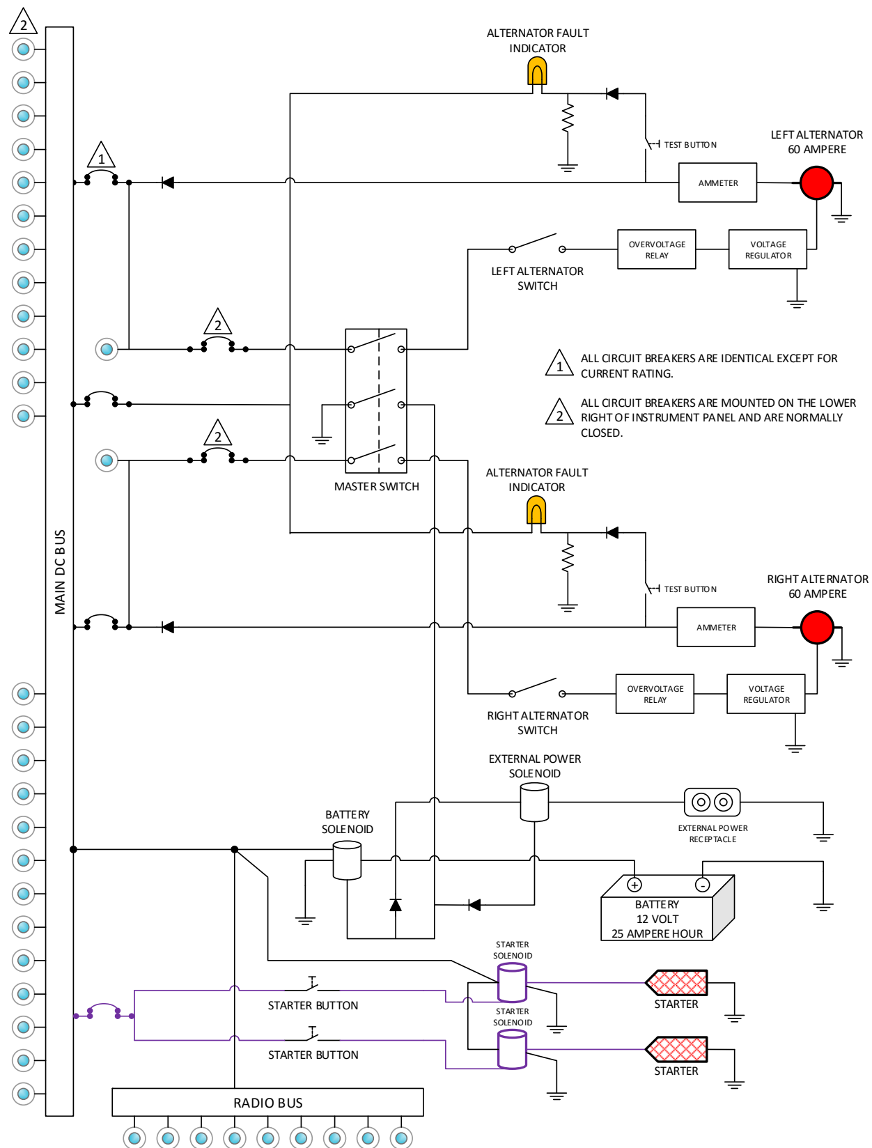
Figure 7-12. Electrical System Schematic.
