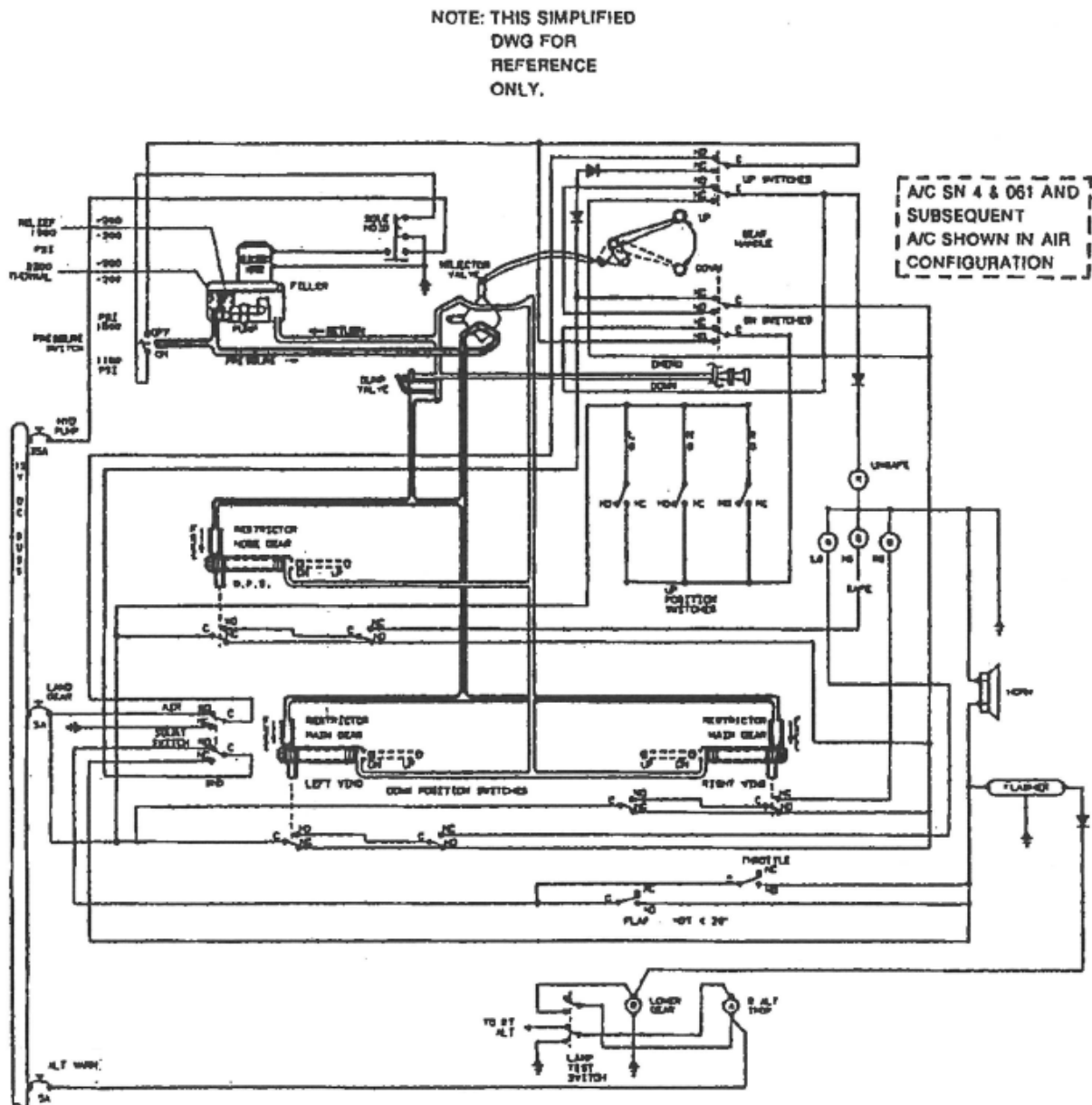
Figure 7-11A. Hydraulic System Schematic (Gear Retracted).
