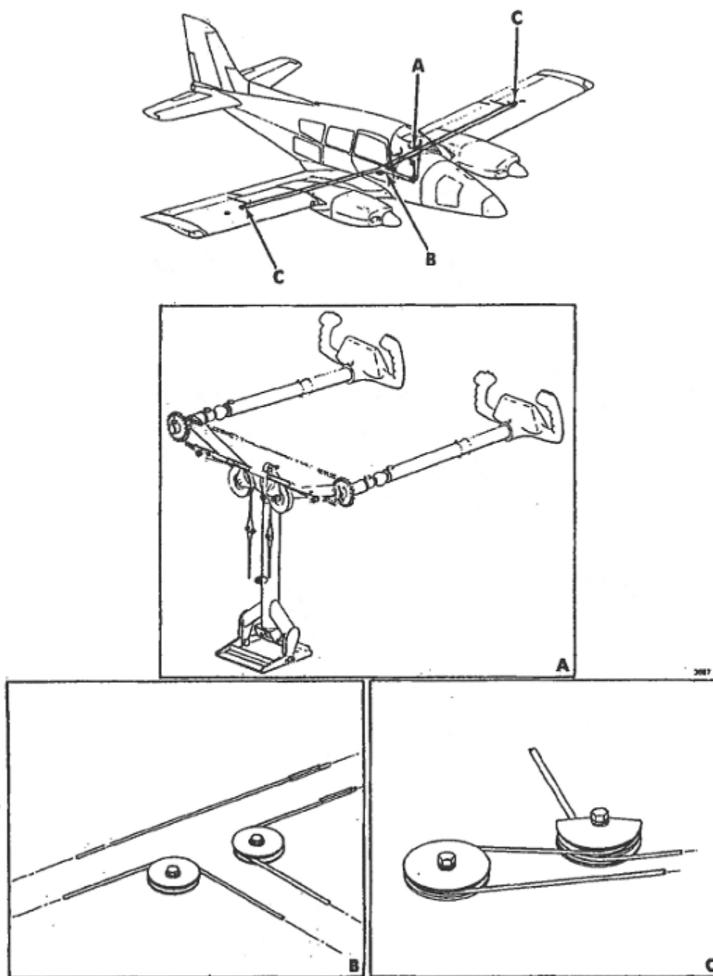
Figure 7-1. Aileron Control System (Sheet 1 of 2)
