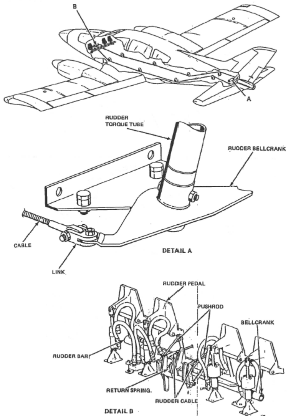
Figure 7-4. Rudder Control System.
