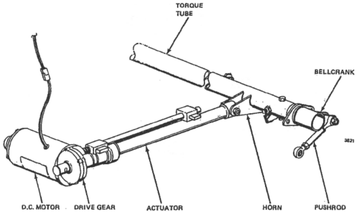
Figure 7-6. Flap Drive Mechanism.
