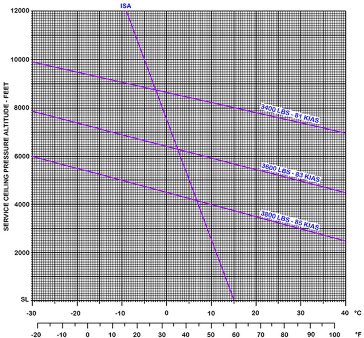
Figure 5-9. One Engine Inoperative Service Ceiling.
